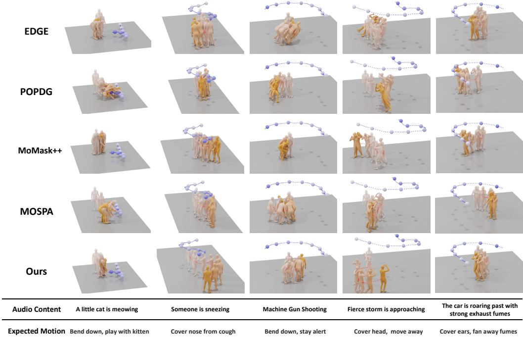
Figure 6: Qualitative comparison of state-of-the-art methods for the dynamic spatial audio-to-motion task. We visualize motion results from five cases.
