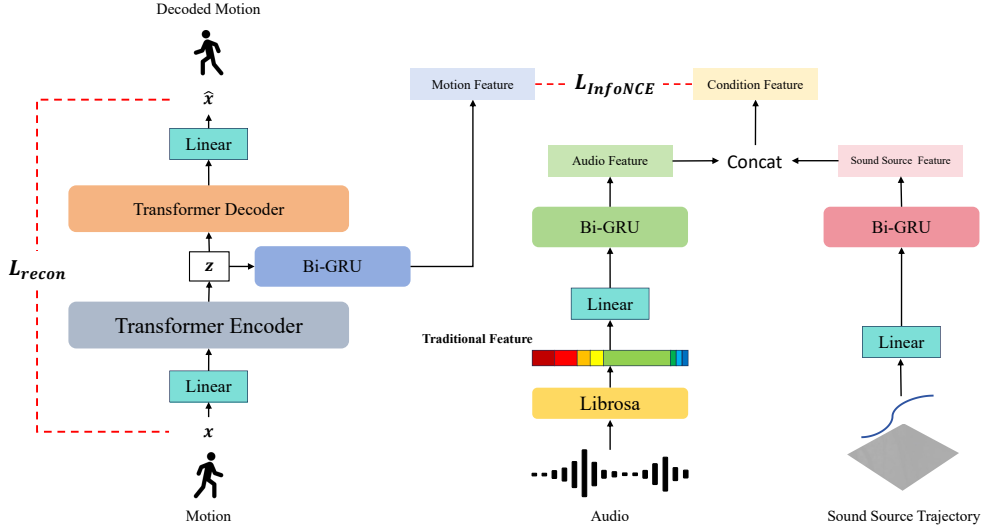
Figure C2: The evaluator framework consists of a motion autoencoder co-trained with Bi-GRU feature extractors. A reconstruction loss \mathcal{L}_{\text{recon}} is applied between the ground-truth motion \mathbf{x} and the decoded motion \hat{\mathbf{x}} produced by the motion autoencoder. Two Bi-GRU encoders extract the audio feature and the sound source feature from the binaural audio and the sound source trajectory, respectively, and the concatenation of the two features forms the condition latent. Additionally, an InfoNCE loss \mathcal{L}_{\text{InfoNCE}} operates on the extracted condition features and motion features.
