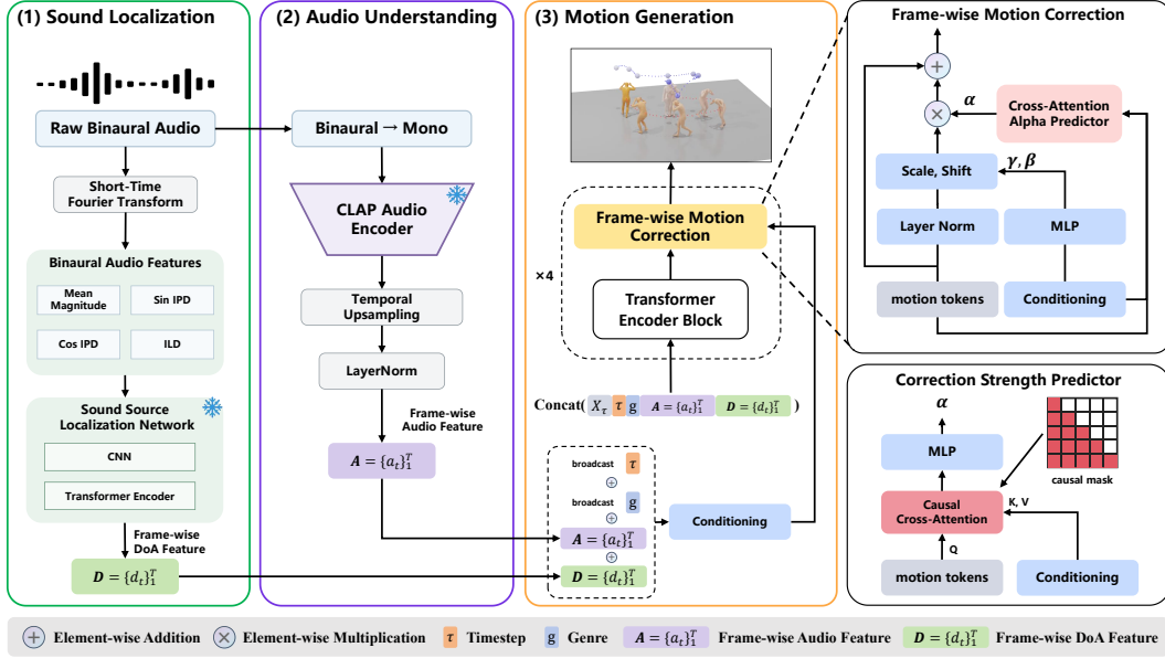
Figure 5: Overview of MOMO framework. MOMO comprises three coupled functional components: a sound source localization (SSL) network predicts a frame-wise head-centric DoA sequence \hat{D} from binaural audio ( localization ); a CLAP audio encoder extracts frame-wise audio content features A from mono audio ( understanding ); and a conditional diffusion model that iteratively denoise the Gaussian noise to generated motion, integrating Frame-wise Motion Correction to adaptively correct each motion according to frame-wise conditions ( generation ).
